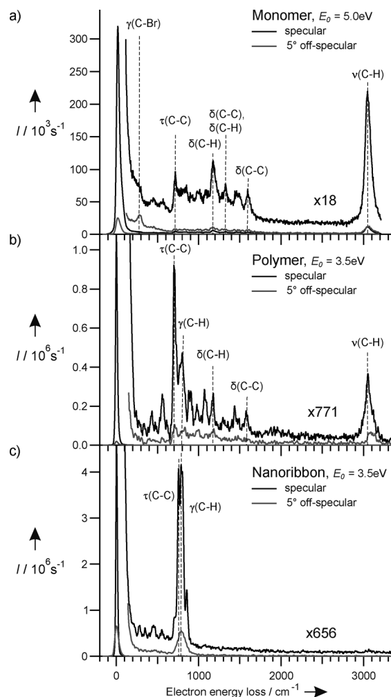
Figure 1. On-surface synthesis of the undoped GNR analyzed by vibrational HREELS in specular and off-specular scattering geometry for the three reaction steps: a) adsorbed monomers, b) polymer and c) graphene nanoribbon. E_0 is the primary energy of the incident electrons.
